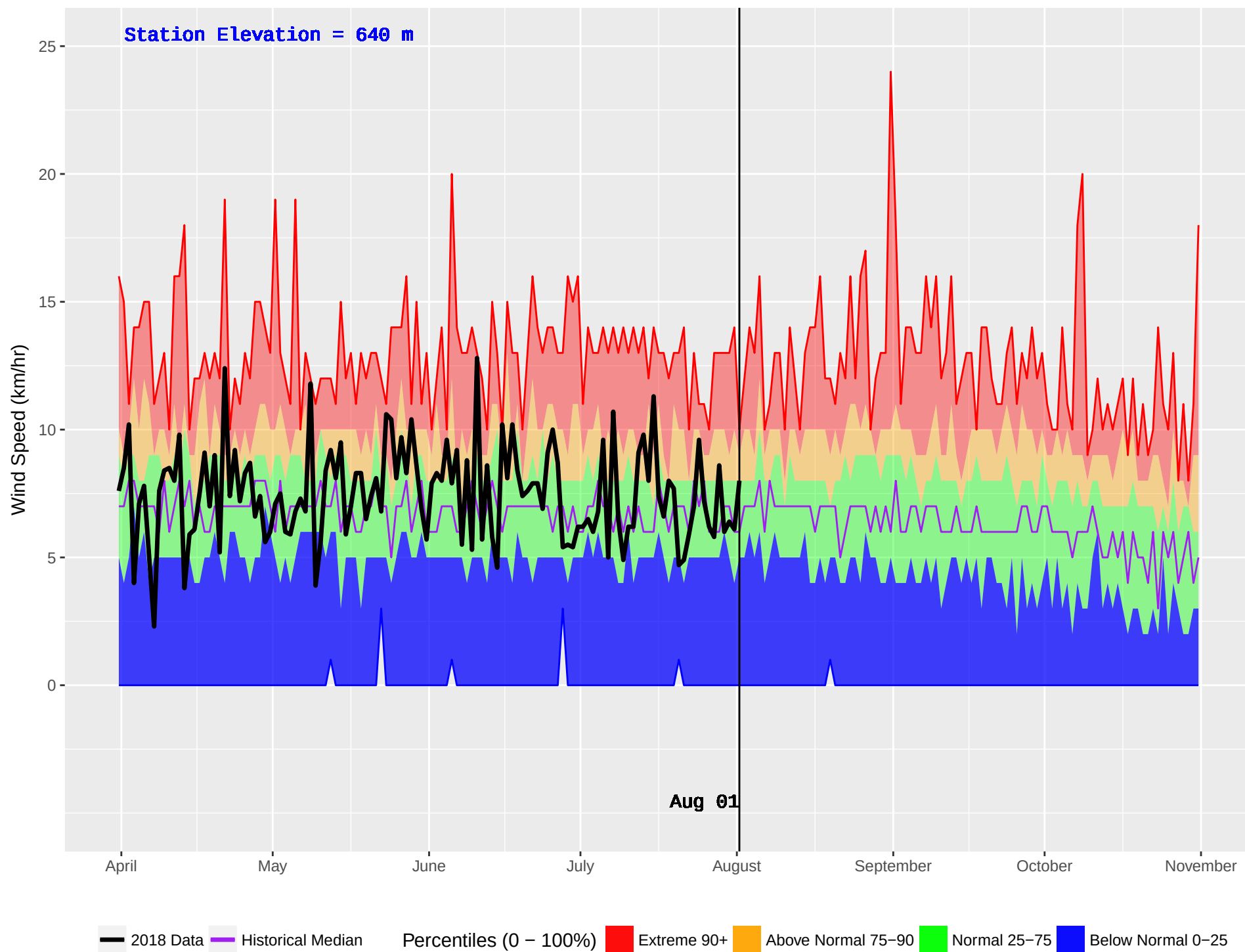
TURTLE (286) : Historical (1977–2016) and Current (2018) Daily Wind Speed
